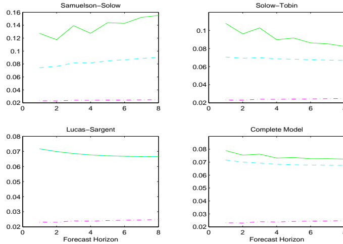
Figure 11: Optimal Policy v. Zero Inflation, 1992.Q4
