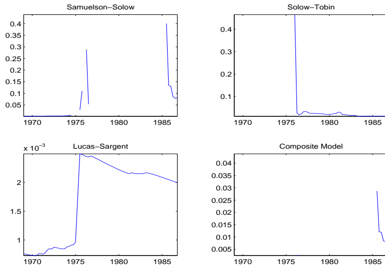
Figure 3: Expected Loss of a Zero Inflation Policy.
