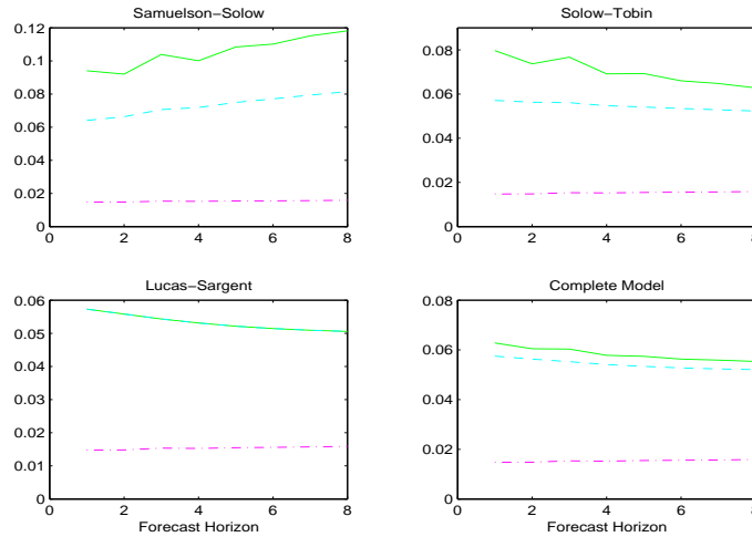
Figure 12: Optimal Policy v. Zero Inflation, 2002.Q4
