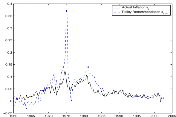
Figure 2: Inflation and Optimal Policy
