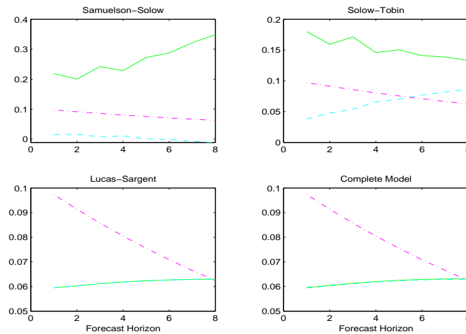
Figure 6: Optimal Policy v. Zero Inflation, 1979.Q4
