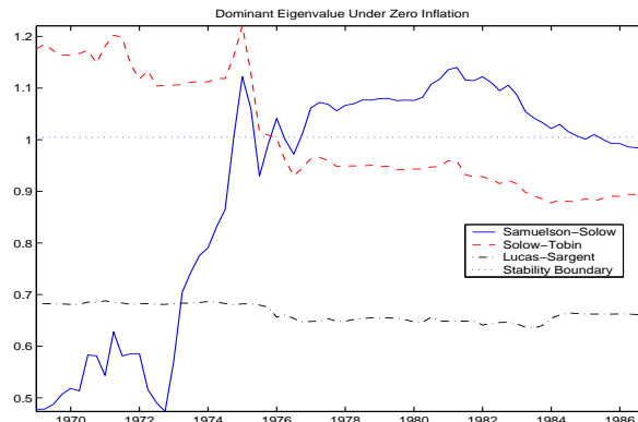
Figure 4: Dominant Eigenvalue Under Zero Inflation
