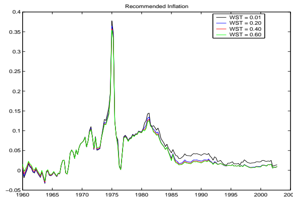
Figure 10: Sensitivity of Bayesian Policy to Prior Model Weights
