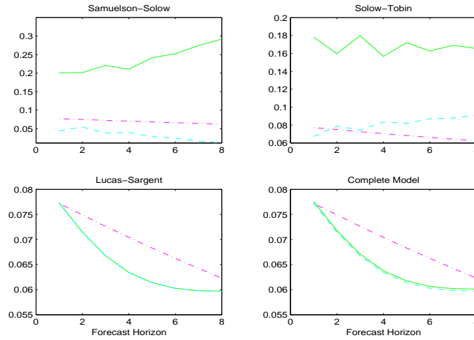
Figure 5: Optimal Policy v. Zero Inflation, 1975.Q4
