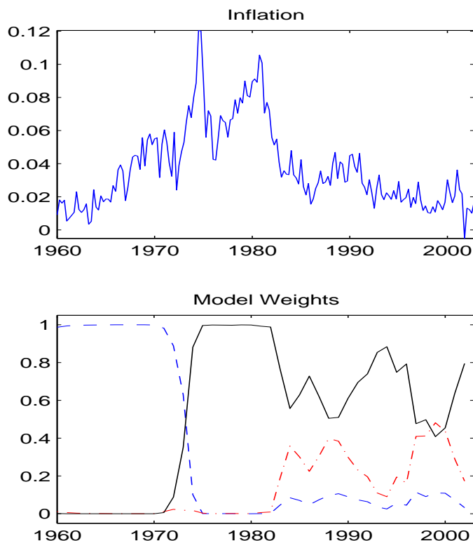
Figure 1: Inflation and Posterior Model Probabilities
