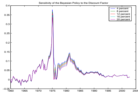
Figure 8: Sensitivity of Bayesian Policy to the Discount Factor
