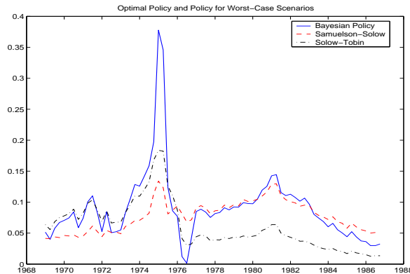
Figure 7: Optimal Policy and Policy for Worst-Case Scenarios
