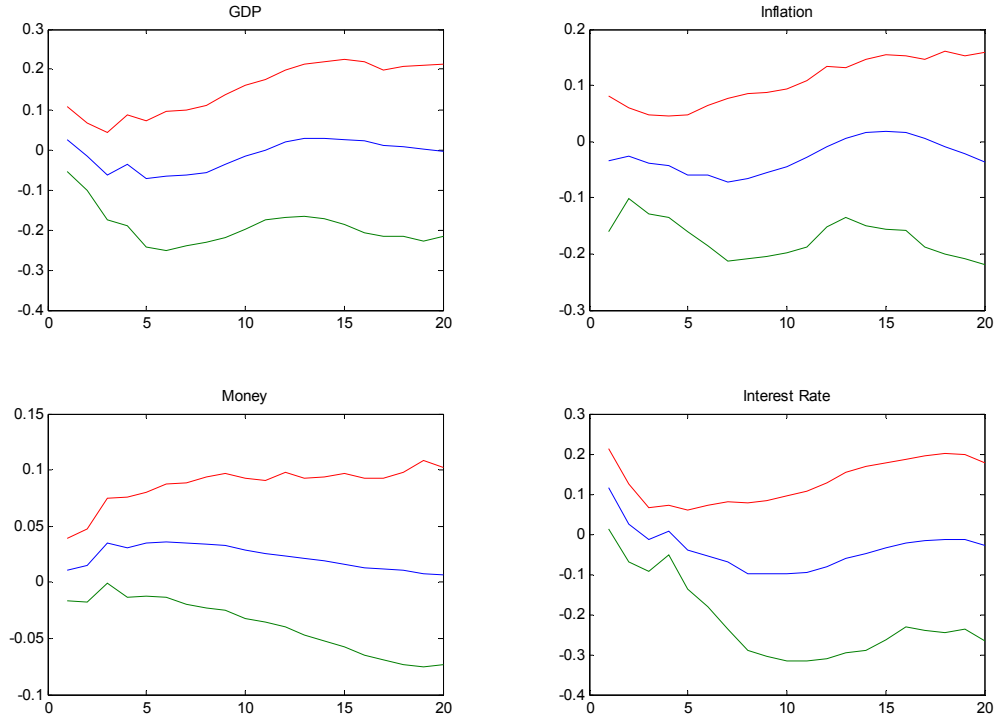
Posterior means and 68% bands of difference in impulse response functions (83-96)
