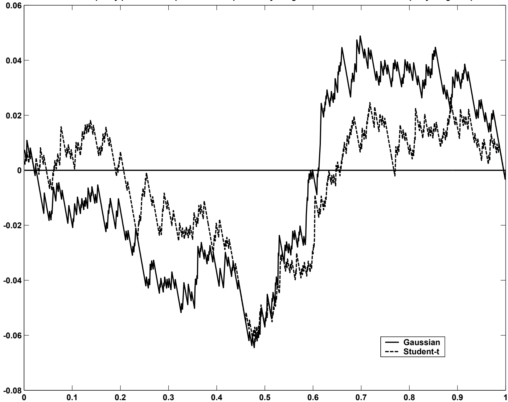
FIGURE 7: Discrepancy plot of the empirical c.d.f. of probability integral transform of returns on equally weighted portfolio
