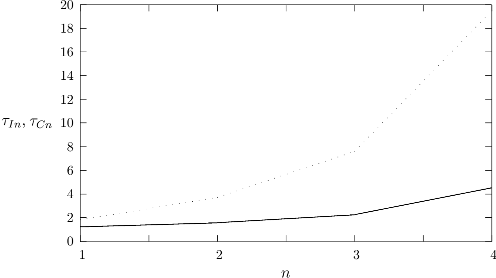
Figure 2: Comparing price informativeness with a single, risk-neutral insider (continuous line) and with a monopolistic information seller (dotted line), when \tau_v = \tau_u = \gamma = 1 and N = 4 .
