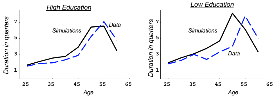
Figure 5: Actual and Fitted Mean Durations by Education
