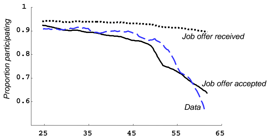
Figure 2: Actual and fitted participation profiles for the low education group
