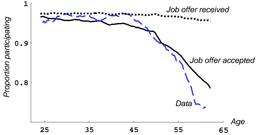
Figure 3: Actual and fitted participation profiles for the high education group
