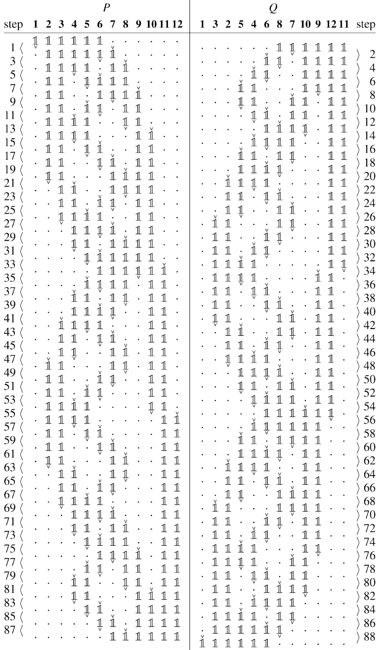
FIGURE 3.—The path A(6) = \pi(6, 1) .
