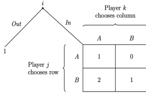
Figure 2: A three-person game form
