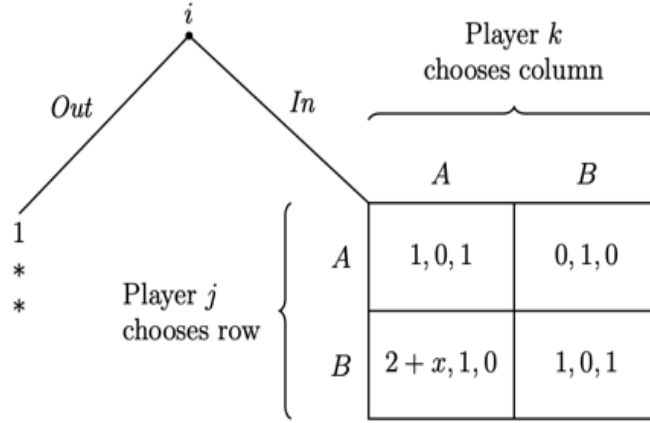
Figure 8: A parameterized three-person game form
