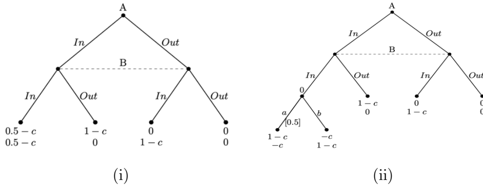
Figure 15: Two market-entry game forms
