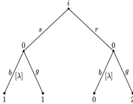
Figure 6: Chance is a follower with perfect information
