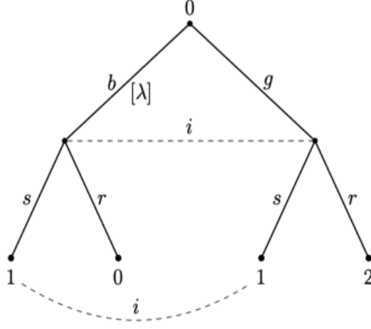
Figure 5: A one-person essentially simultaneous game form with imperfect feedback
