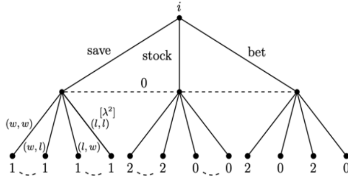
Figure 11: A one-player game form with Chance
