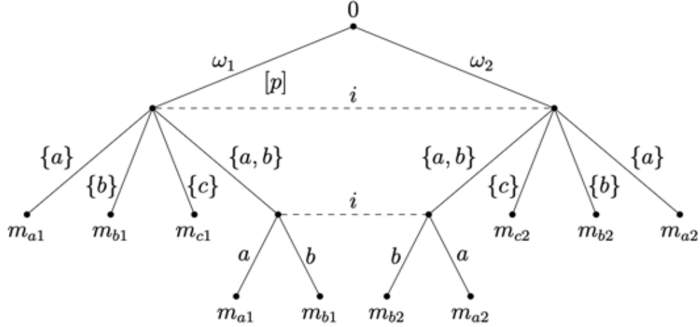
Figure 17: Menu-choice game form
