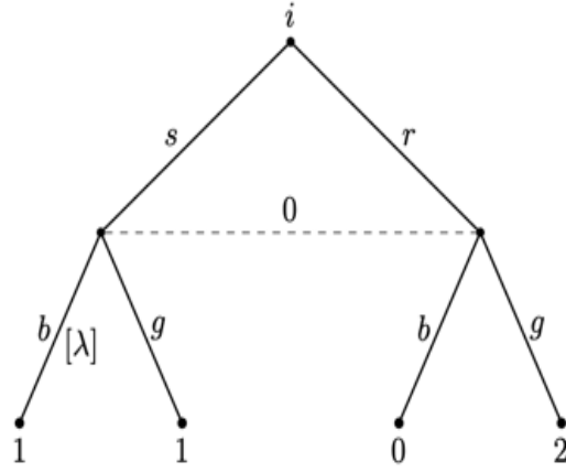
Figure 7: Chance is a follower with imperfect information
