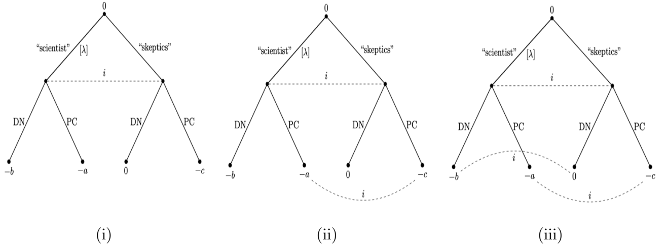
Figure 13: Three climate-action game forms
