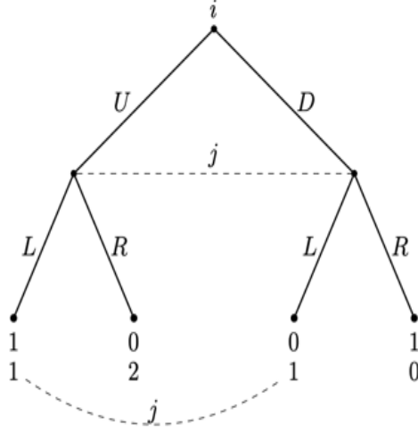
Figure 9: A two-person essentially simultaneous game form with imperfect feedback
