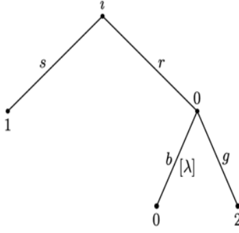
Figure 3: A game form where Chance is a follower
