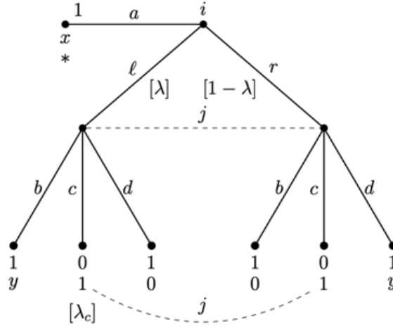
Figure 10: A game form with imperfectly observed actions
