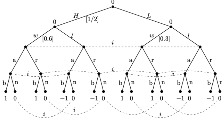
Figure 12: Information acquisition game form
